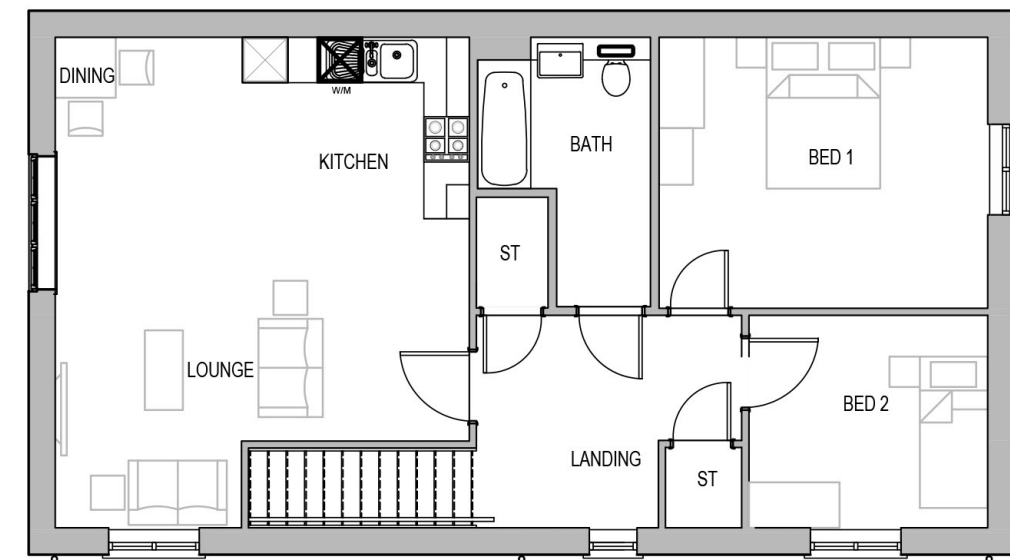
FIRST FLOOR LAYOUT
