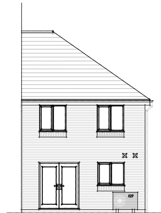
REAR ELEVATION
