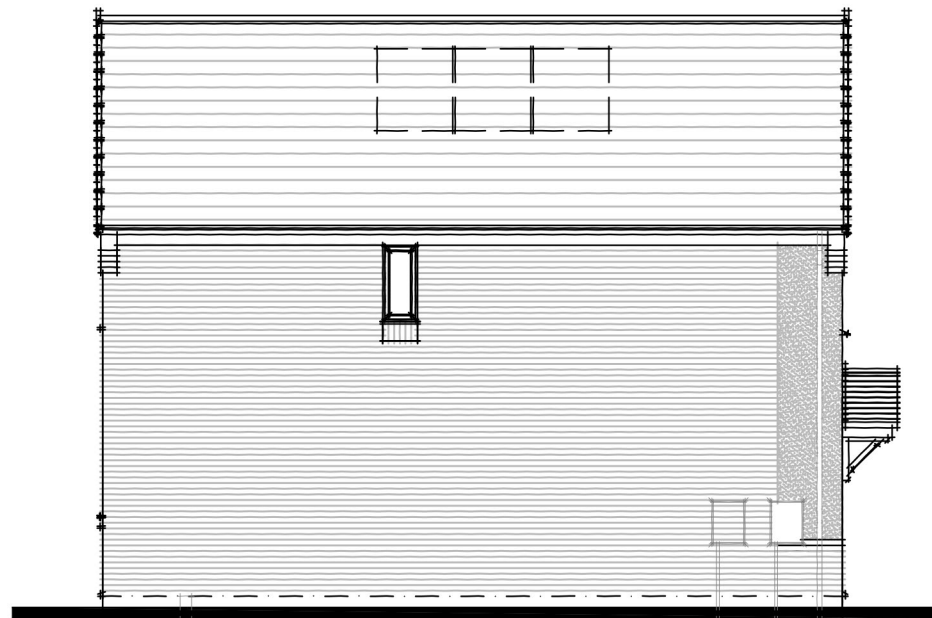
SIDE B ELEVATION
