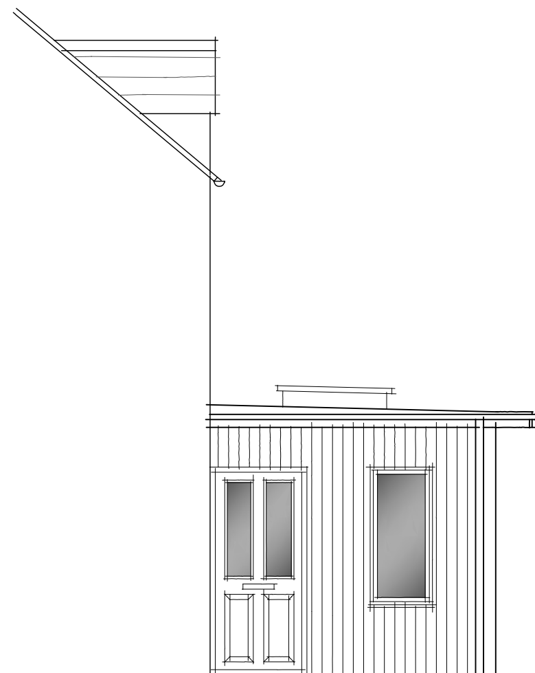
WEST ELEVATION
