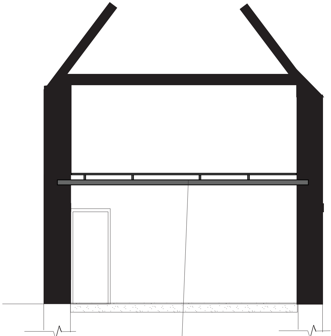
Existing Section C-C Scale 1:50 @ A2
