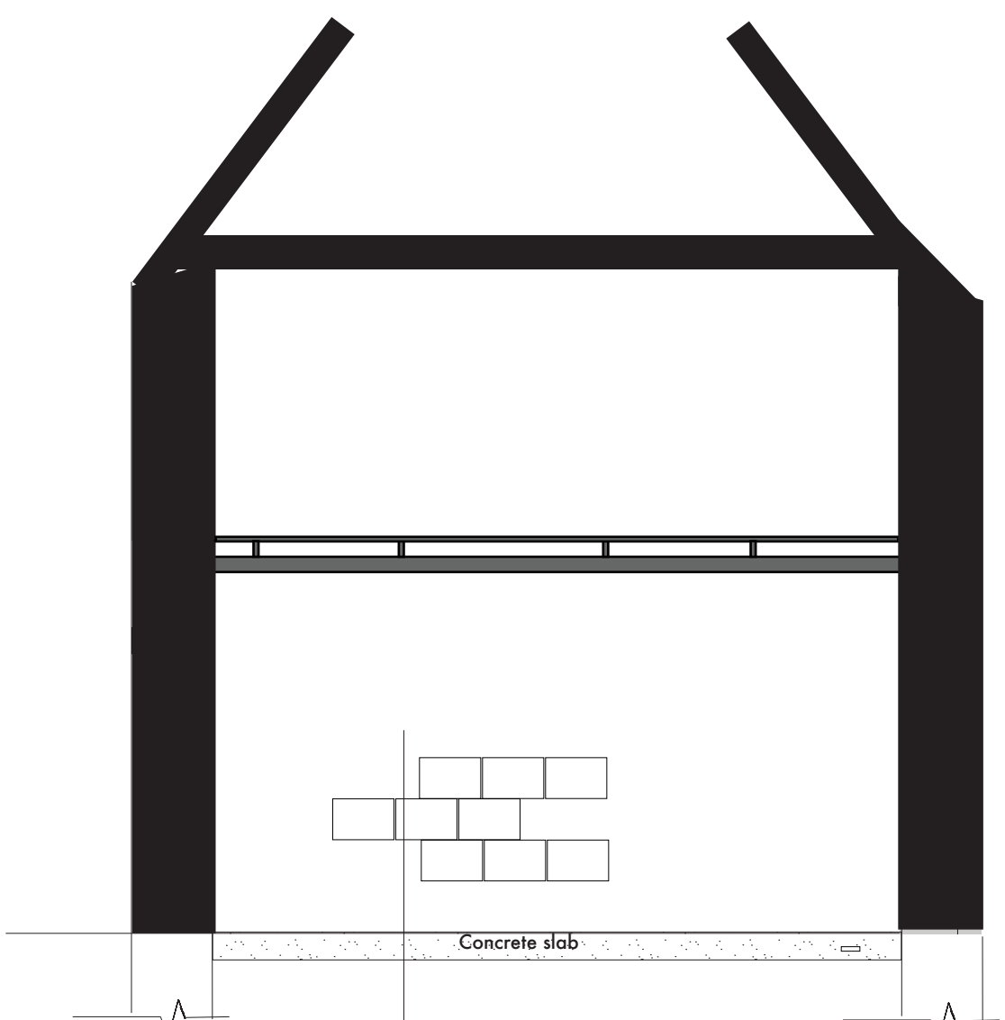
Existing Section D-D Scale 1:50 @ A2
