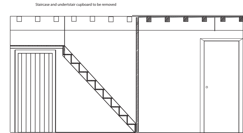
Existing Section B-B Through Kitchen Scale 1:50 @ A2
