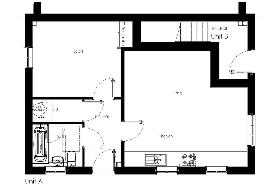
Unit A GROUND FLOOR PLAN
