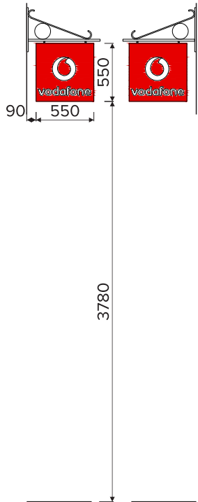
Non illuminated projecting sign 550x550x10mm
