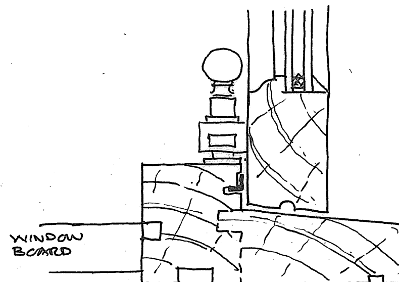
BEAD DETAIL
