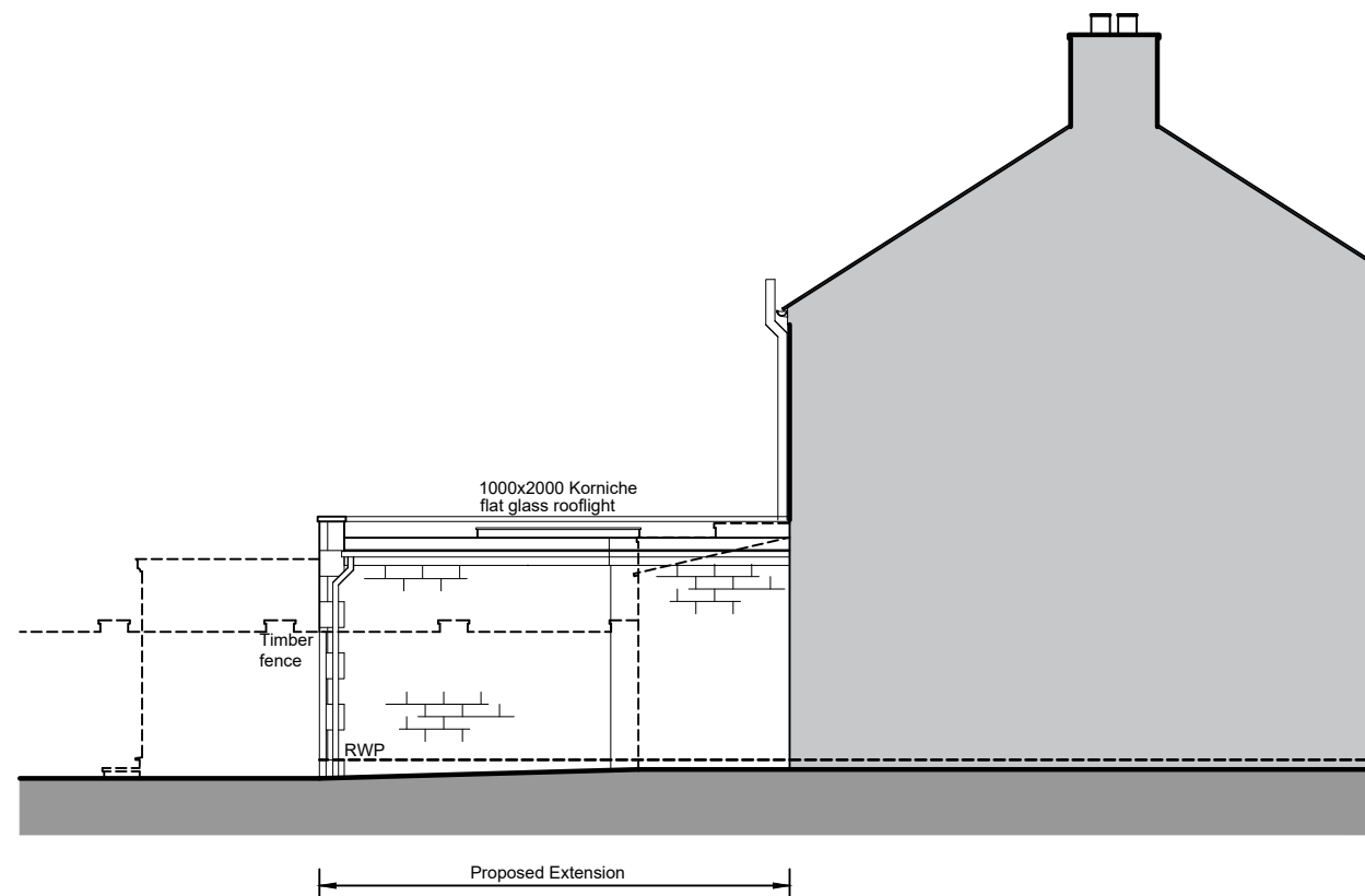
Part South West Elevation
