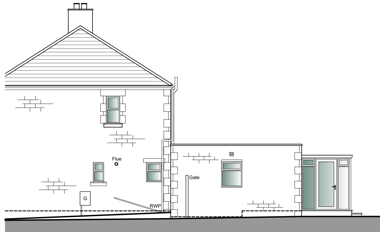
Part North East Elevation
