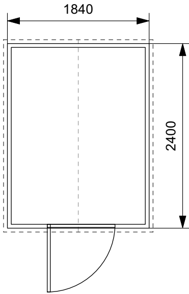
PLAN Scale 1:50
