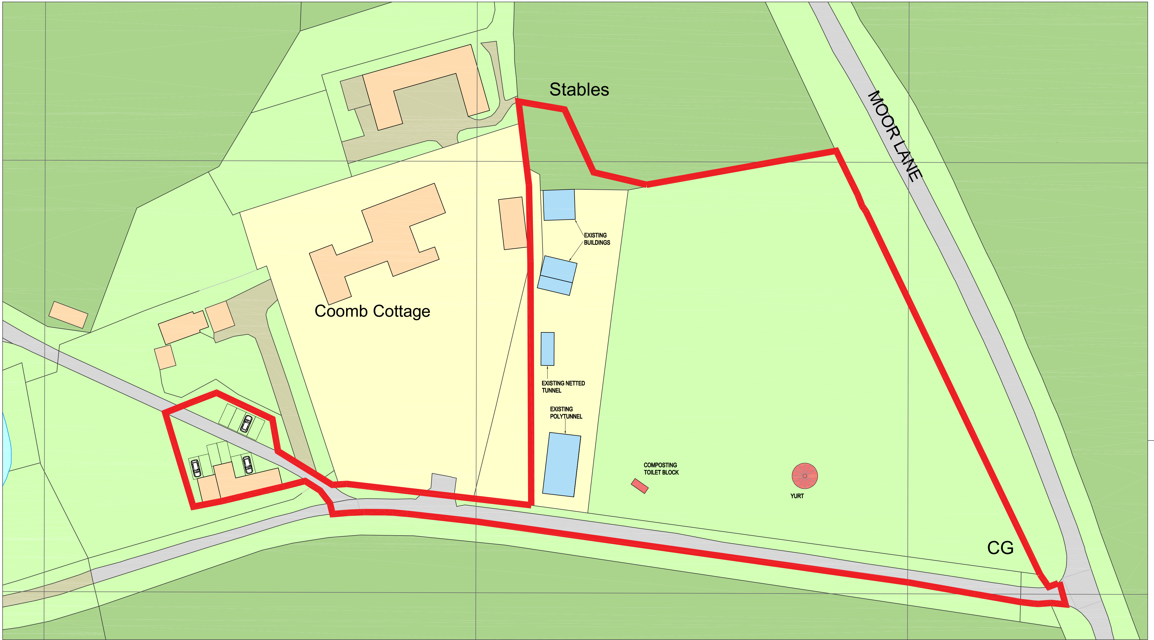
BLOCK PLAN AS PROPOSED 1:500
