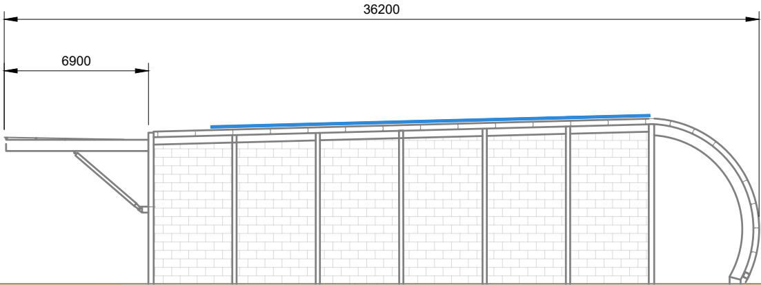
PROPOSED SITE ELEVATION C
