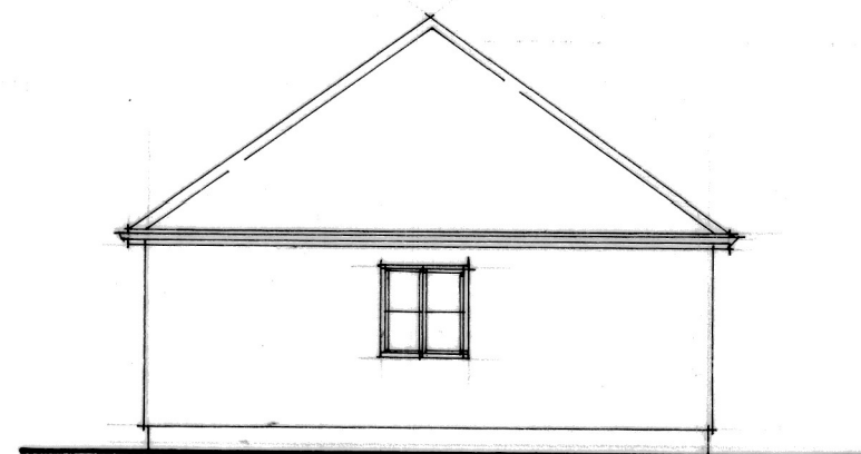
SOUTH ELEVATION
