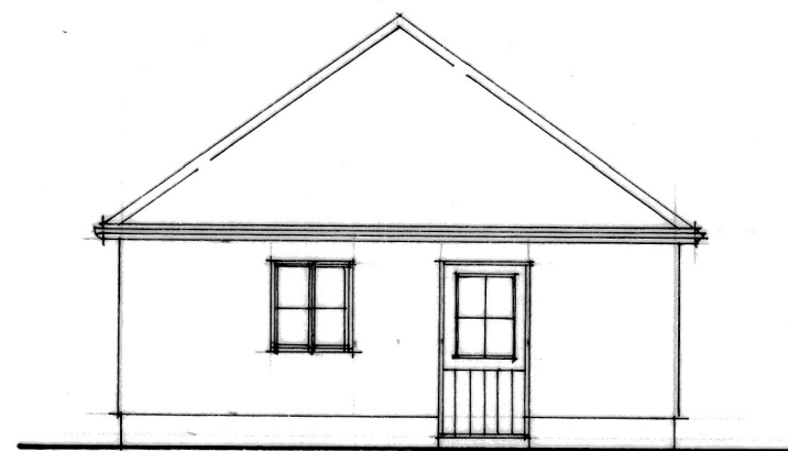
NORTH ELEVATION
