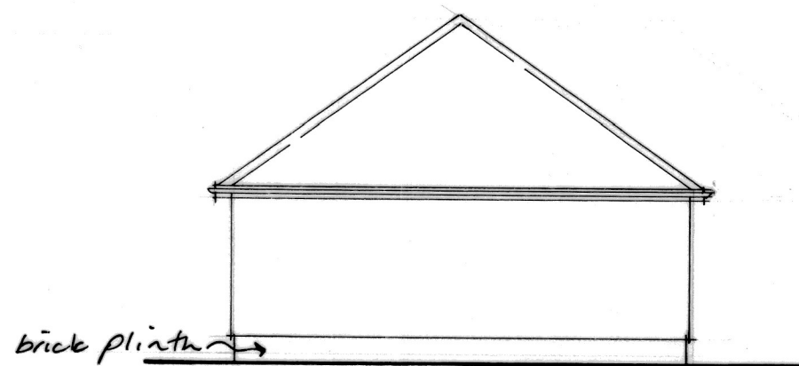
WEST ELEVATION
