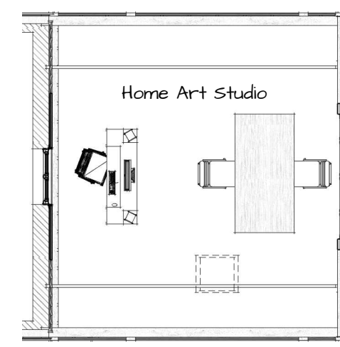
Proposed First Floor
