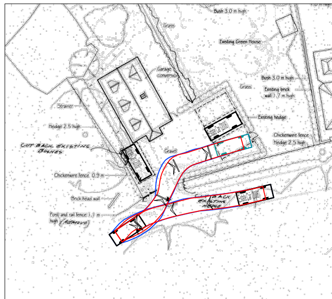
ESTATE CAR ENTERING SPACE 3 MANOEUVRE
