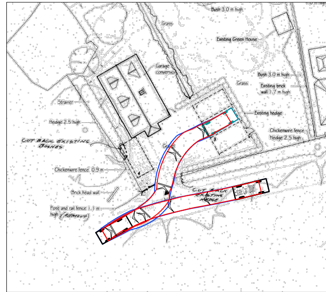
ESTATE CAR ENTERING SPACE 2 MANOEUVRE
