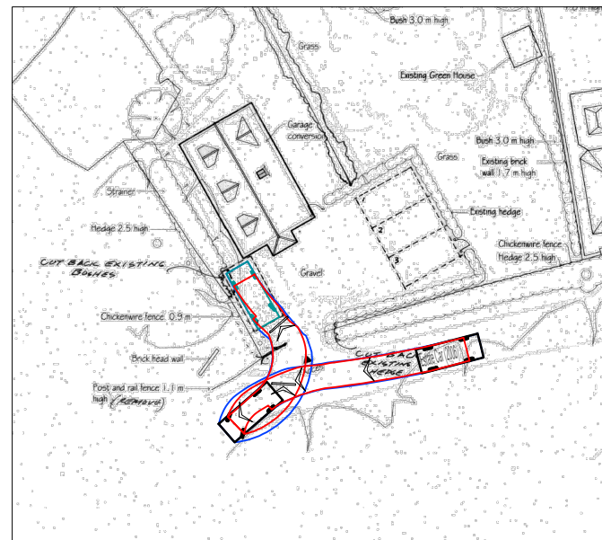
ESTATE CAR ENTERING SPACE 4 MANOEUVRE
