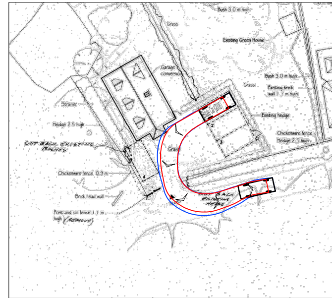
ESTATE CAR EXITING SPACE 1 MANOEUVRE
