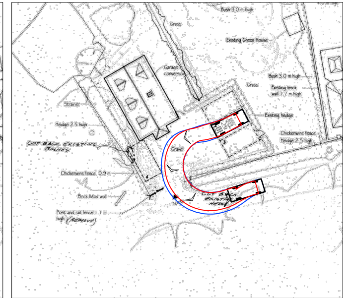
ESTATE CAR EXITING SPACE 2 MANOEUVRE
