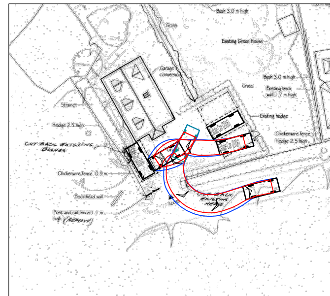
ESTATE CAR EXITING SPACE 3 MANOEUVRE
