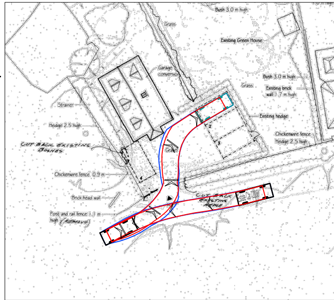
ESTATE CAR ENTERING SPACE 1 MANOEUVRE
