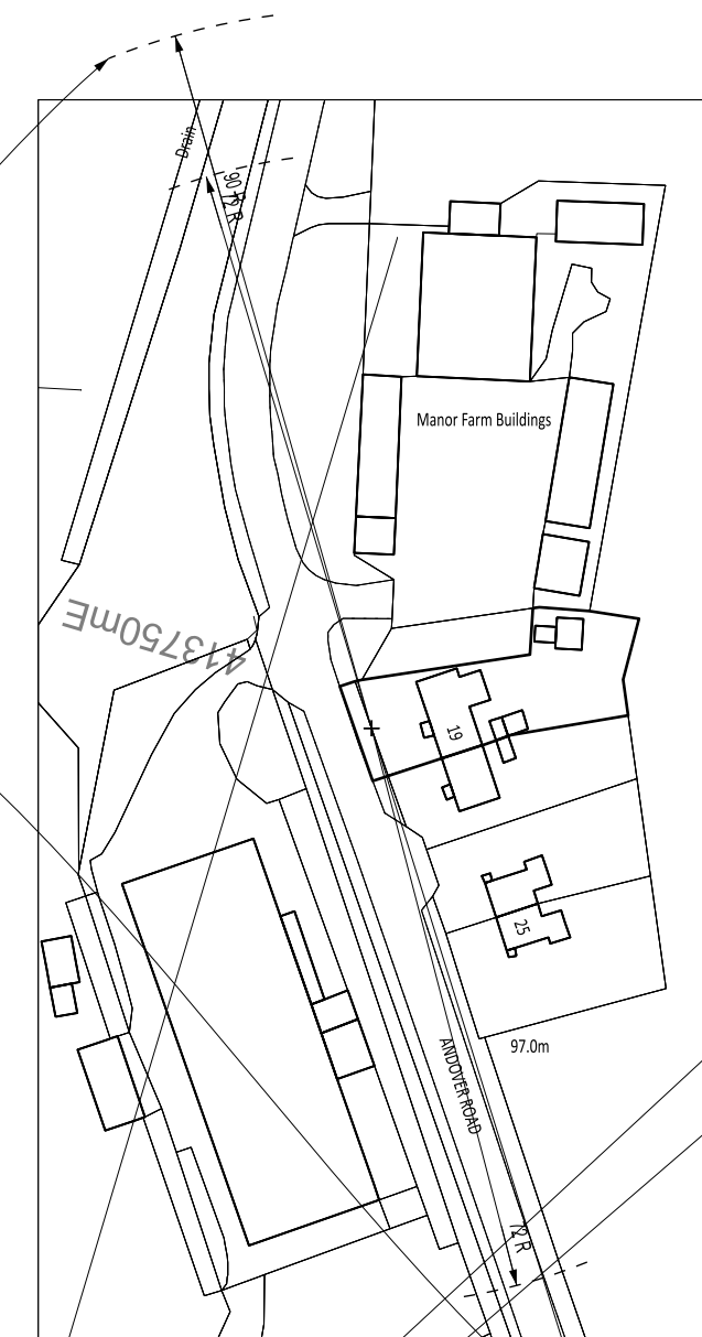
PLAN: LOCATION
