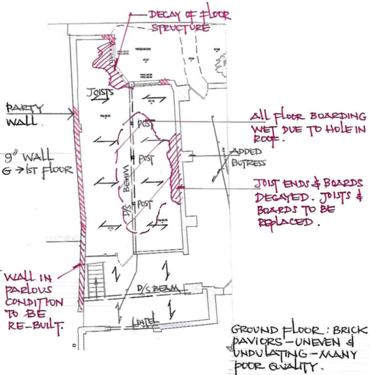
GROUND FLOOR PLAN (FIRST FLOOR STRUCTURE OVER) 1:100
