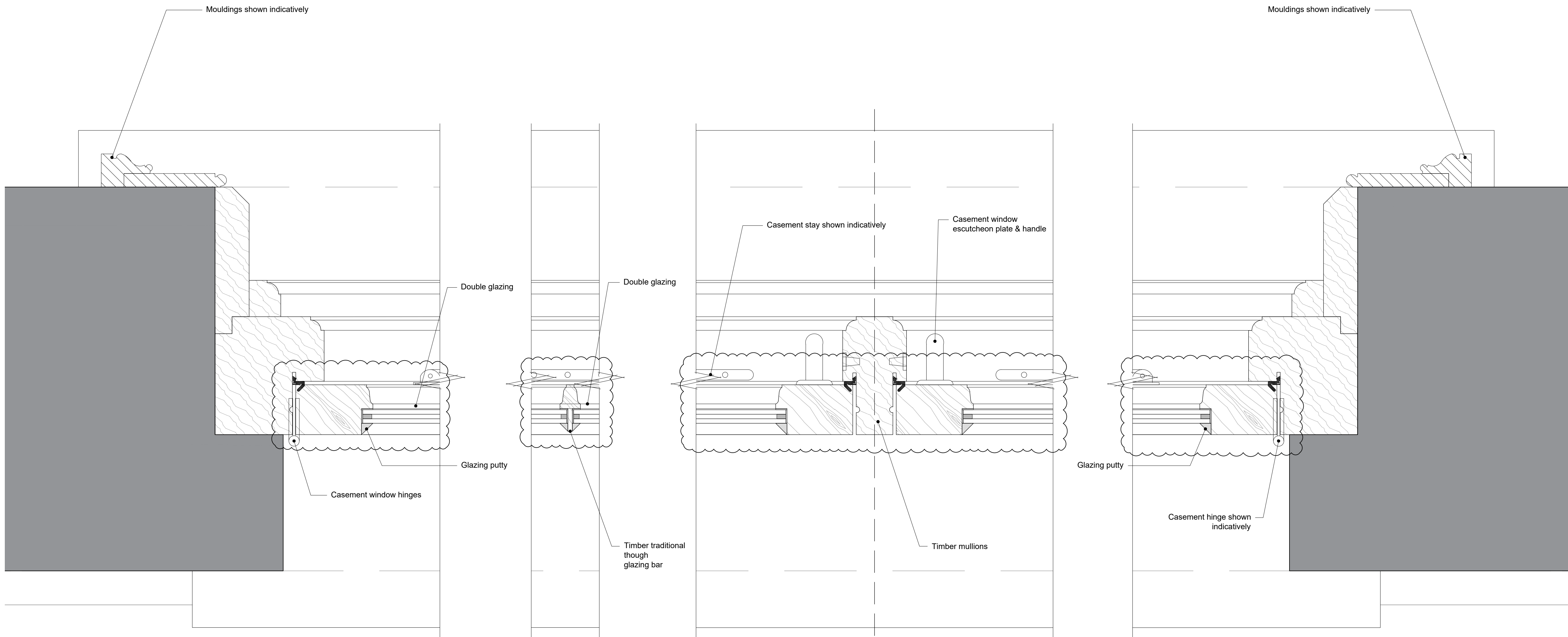
01 Window Type B2 - Jamb Detail 747.3 SCALE 1:2 @ A1
