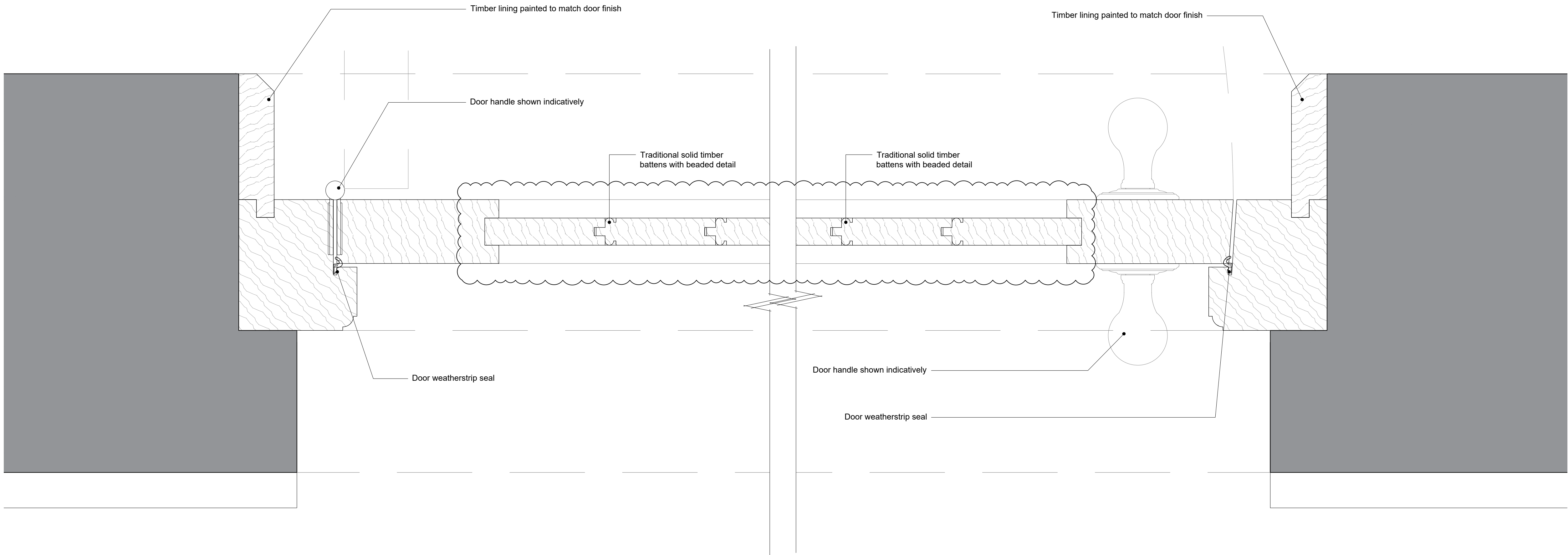
01 Door Type B7 - Timber Framed and Battened Entrance Door Jamb Detail 761.2 SCALE 1:2 @ A1
