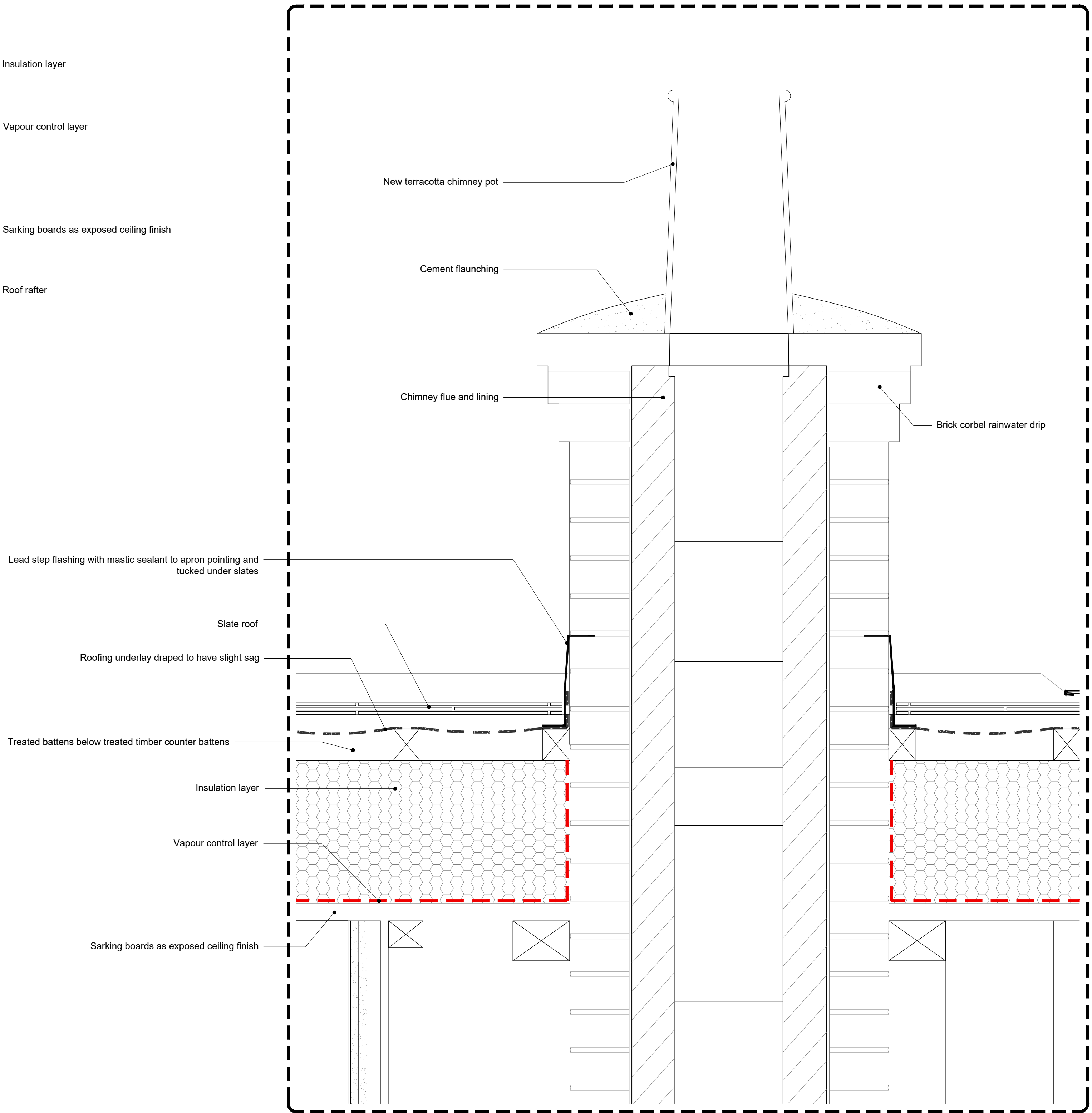
02 Typical Chimney Junction Detail 802.1 SCALE 1:5 @ A1
