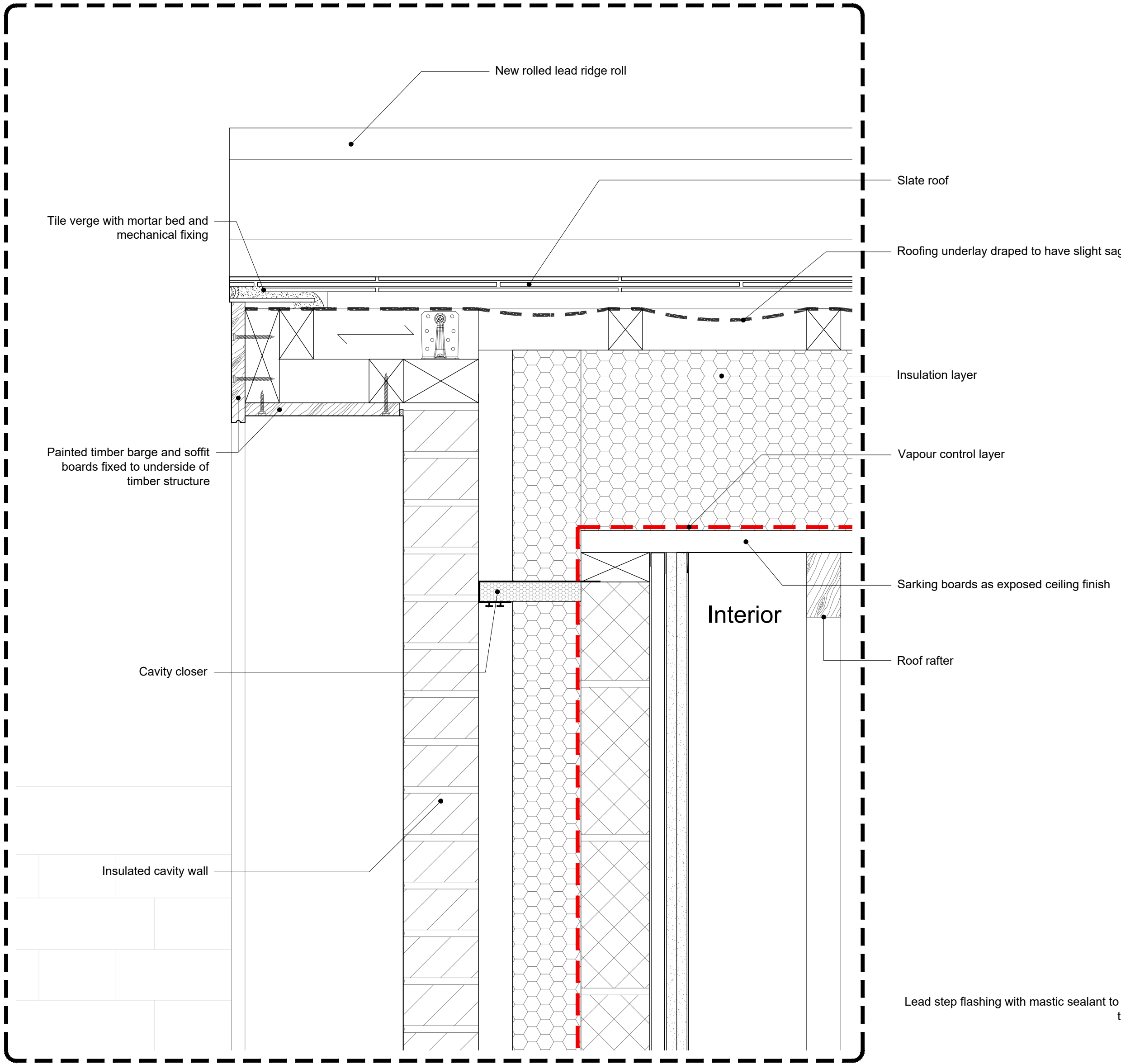
01 Typical Slate Verge Detail 802.1 SCALE 1:5 @ A1
