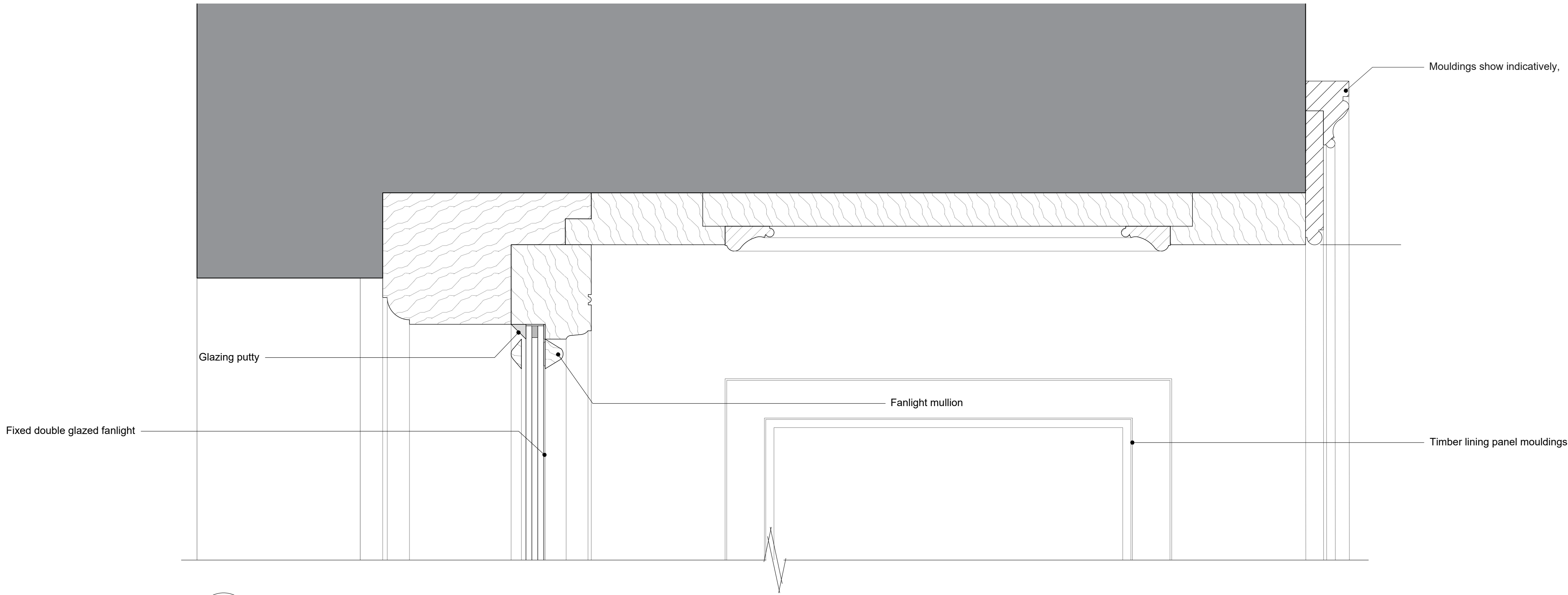
01 Door Type C2 - Fixed Fanlight Head Jamb Detail 765.4 SCALE 1:2 @ A1
