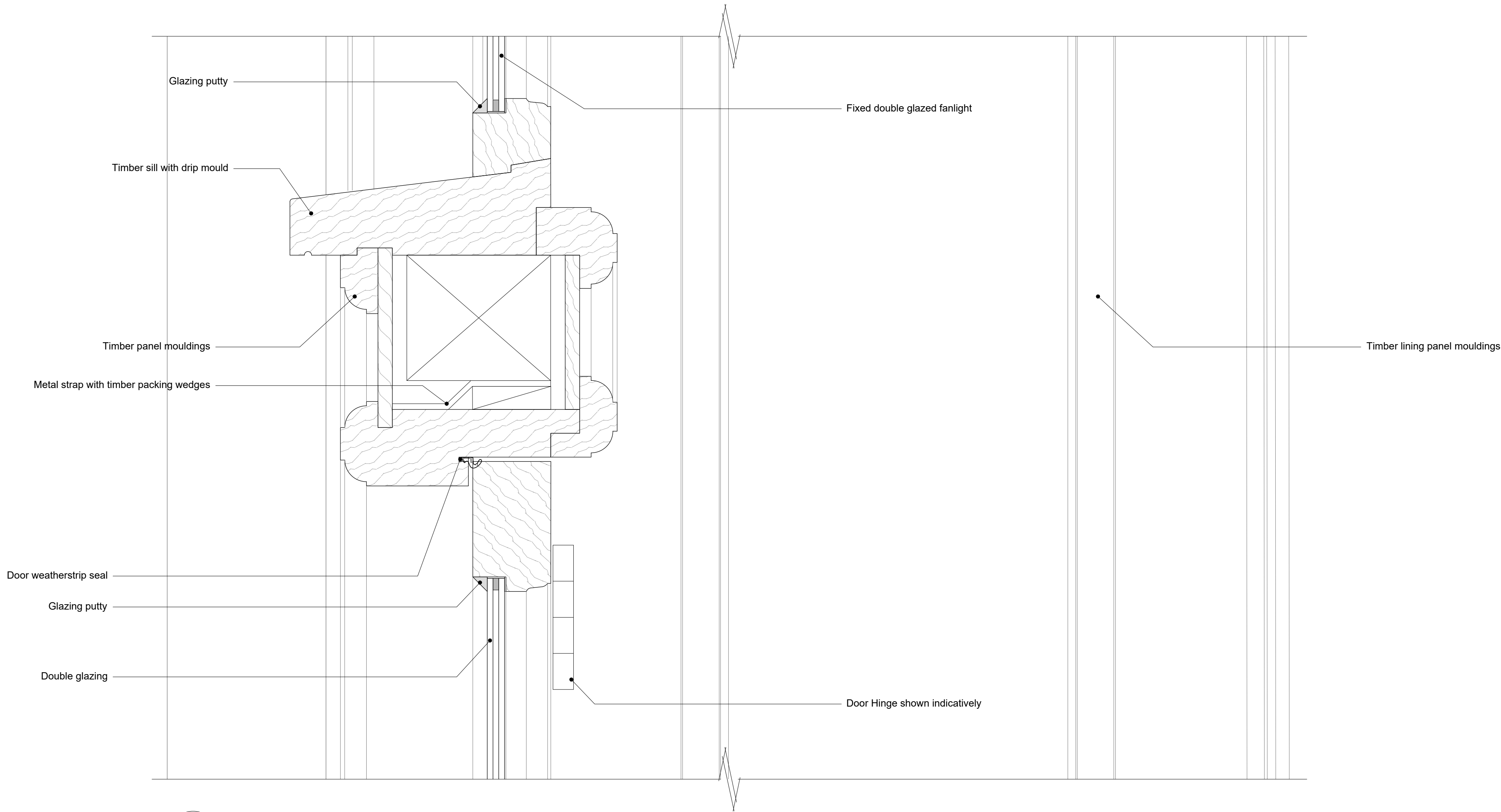
02 Door Type C2 - Fixed Fanlight Sill & French Door Head Jamb Detail 765.4 SCALE 1:2 @ A1
