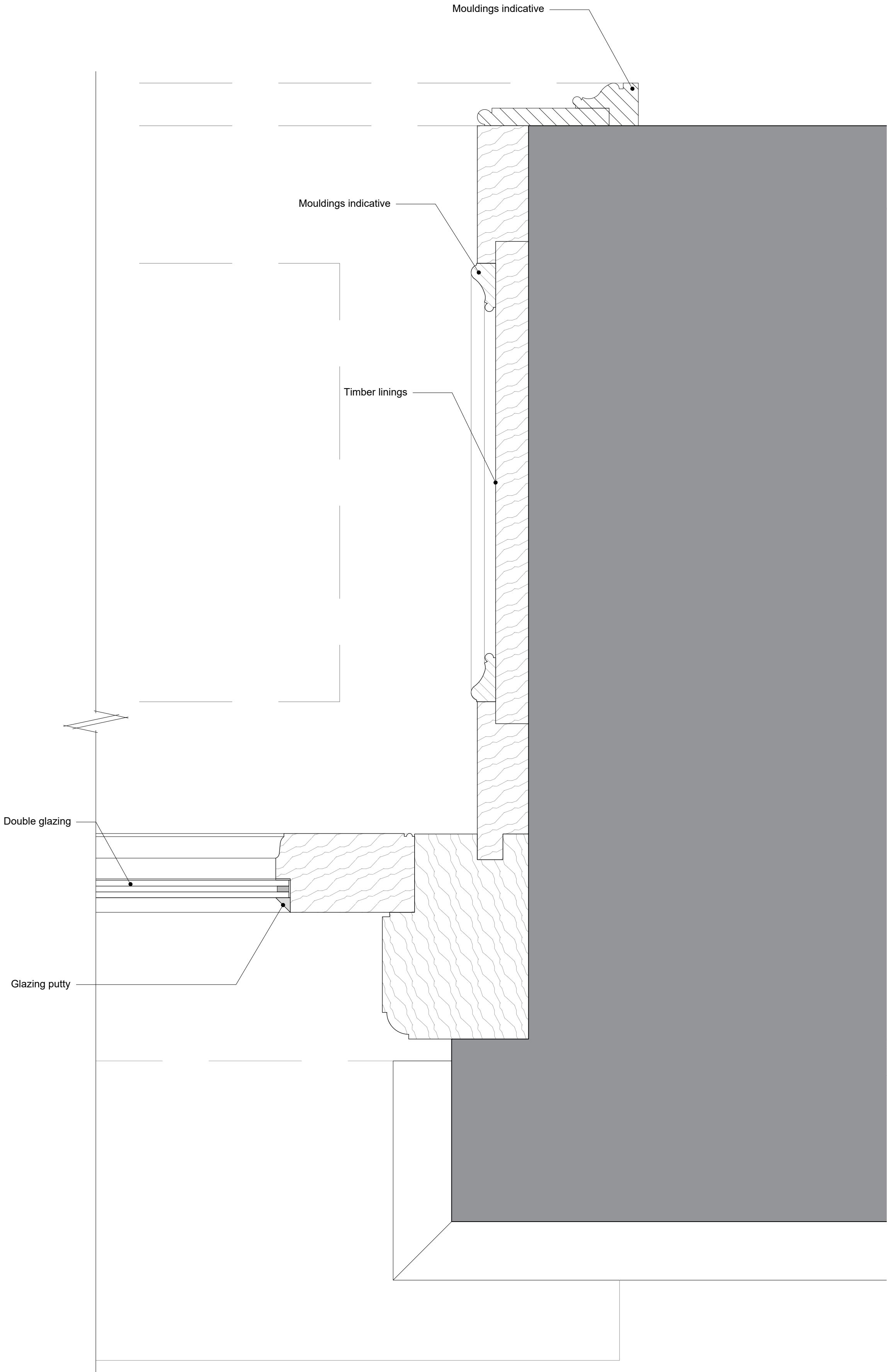
02 Door Type C2 - Fixed Window Jamb Detail 765.3 SCALE 1:2 @ A1
