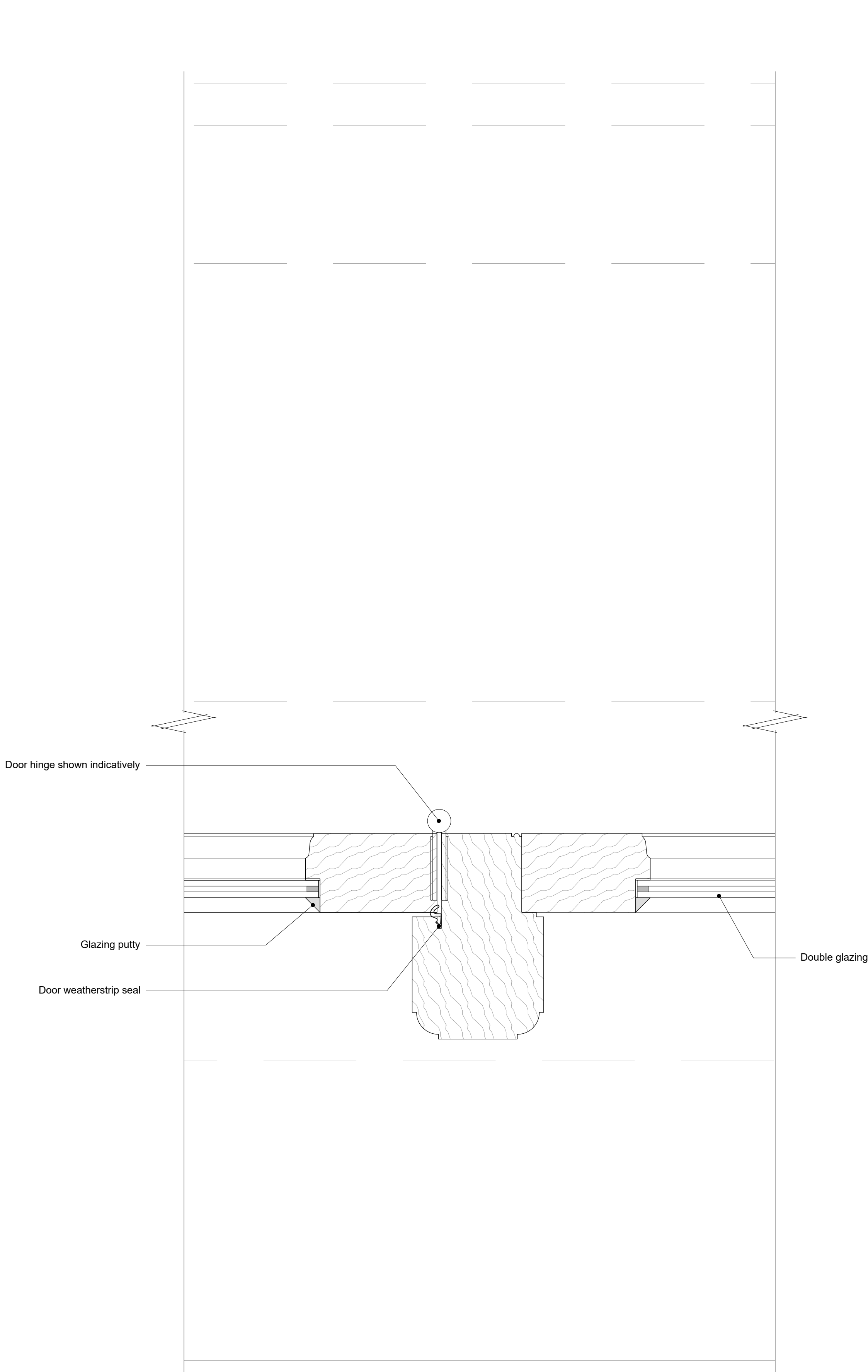
01 Door Type C2 - French Door Hinge Detail 765.3 SCALE 1:2 @ A1
