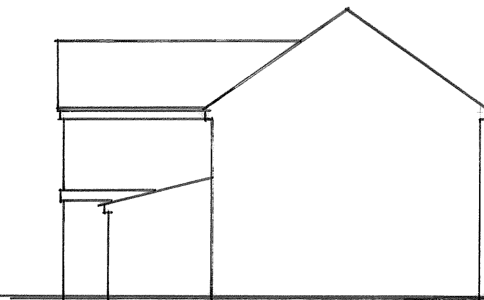
SIDE
