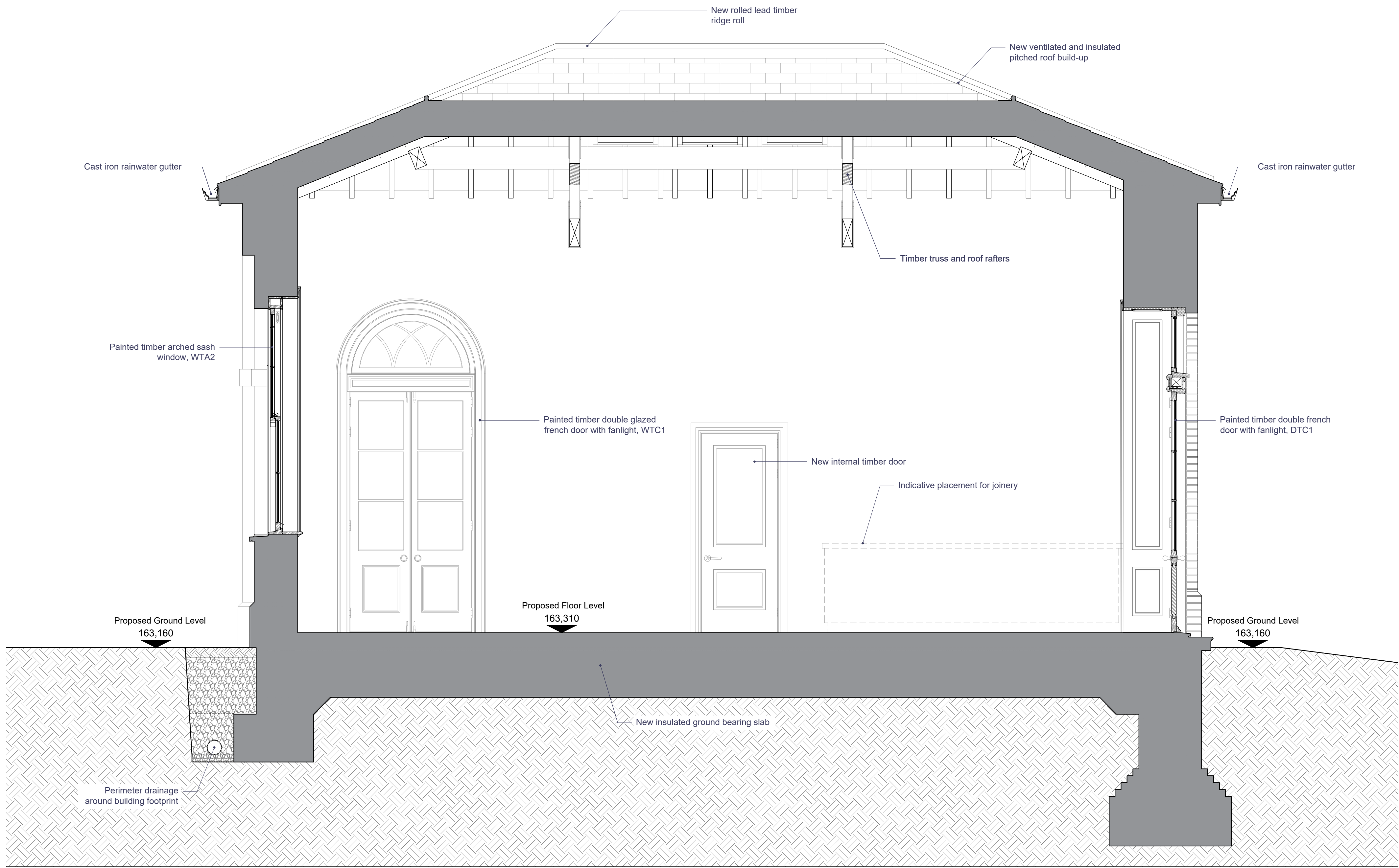
206 Building 5 - Proposed Section A-A 1:25_@_A1
