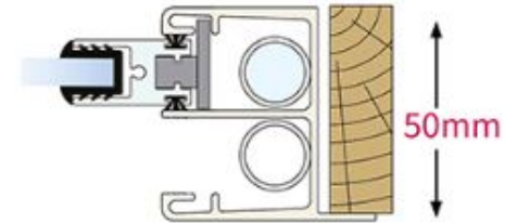
Jamb detail lower sash
