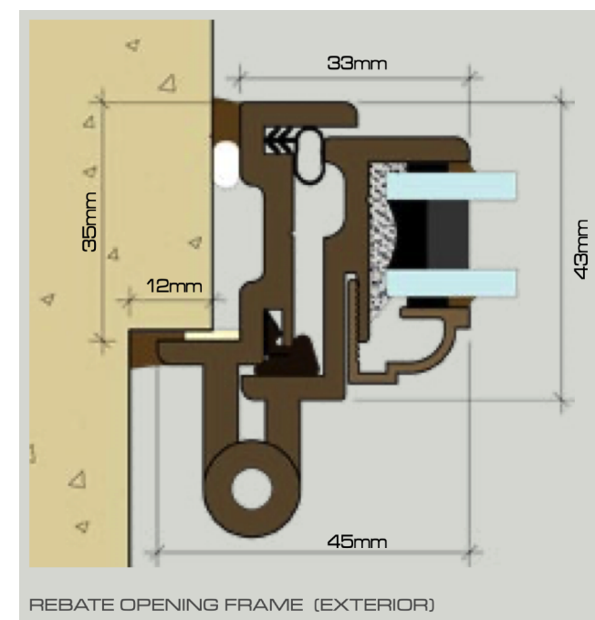
Manufacturers detail for metal window in timber frame
