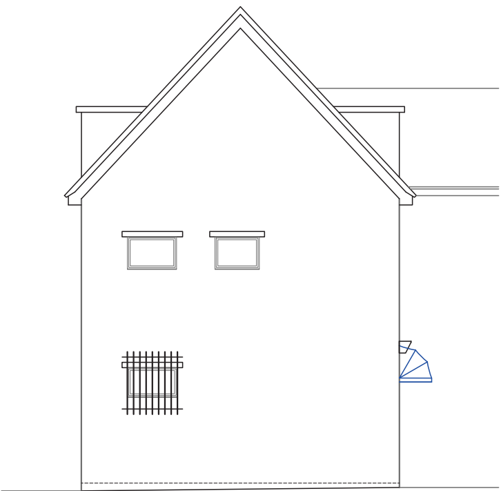
South Elevation
