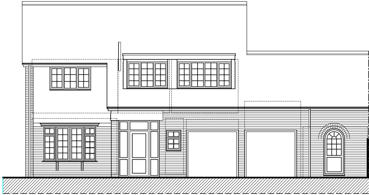
NORTH ELEVATION
