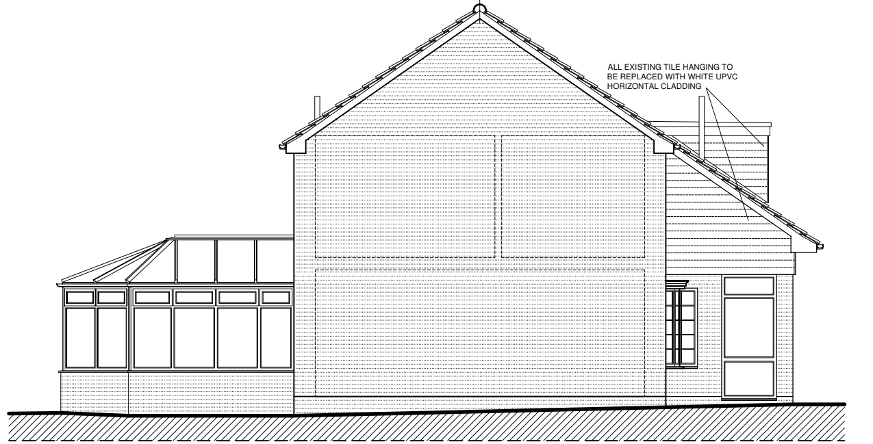
EAST ELEVATION
