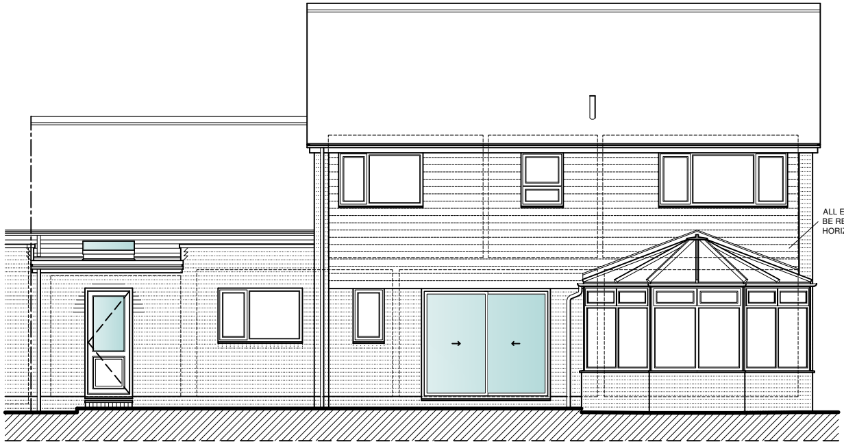
SOUTH ELEVATION
