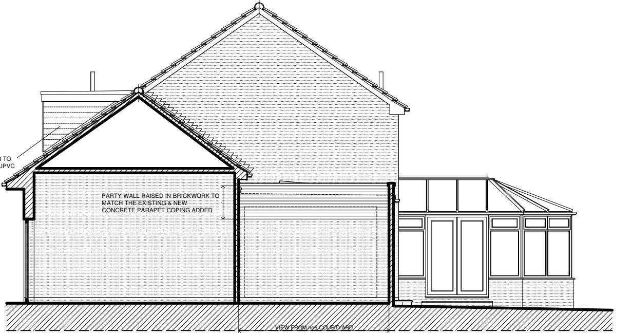
WEST SECTIONAL ELEVATION
