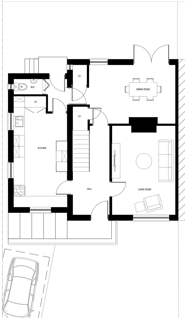
01 -Proposed Ground Floor Plan
