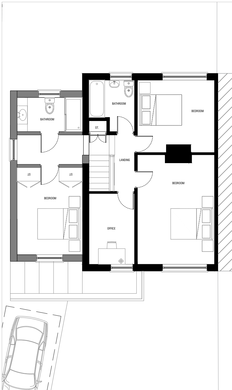
02 -Proposed First Floor Plan
