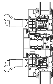
➤ 58BW FLUSH HI MULLION
