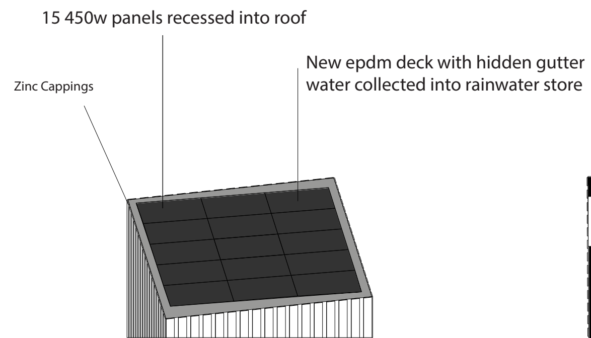
South Elevation
