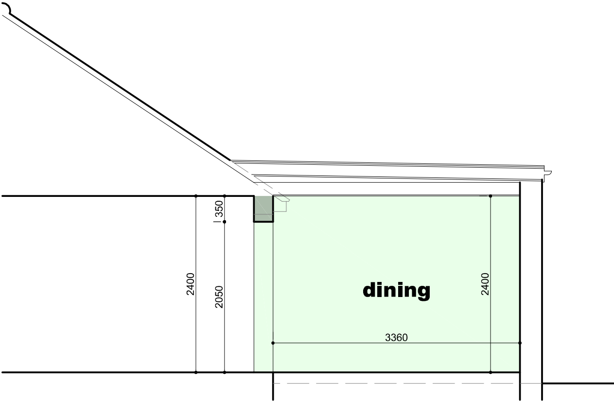
SECTION
