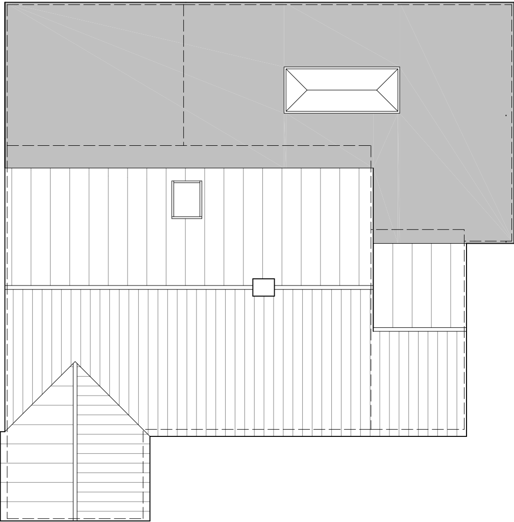
ROOF PLAN
