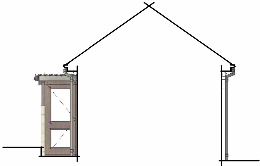
3 Side (North West) Elevation 1 : 50
