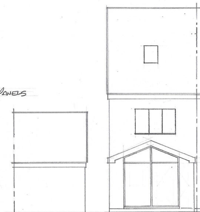
PROPOSED WEST ELEVATION (REAR)
