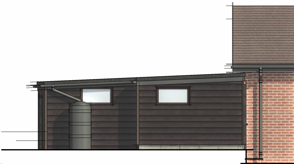
2 Rear (North East) Elevation 1 : 50
