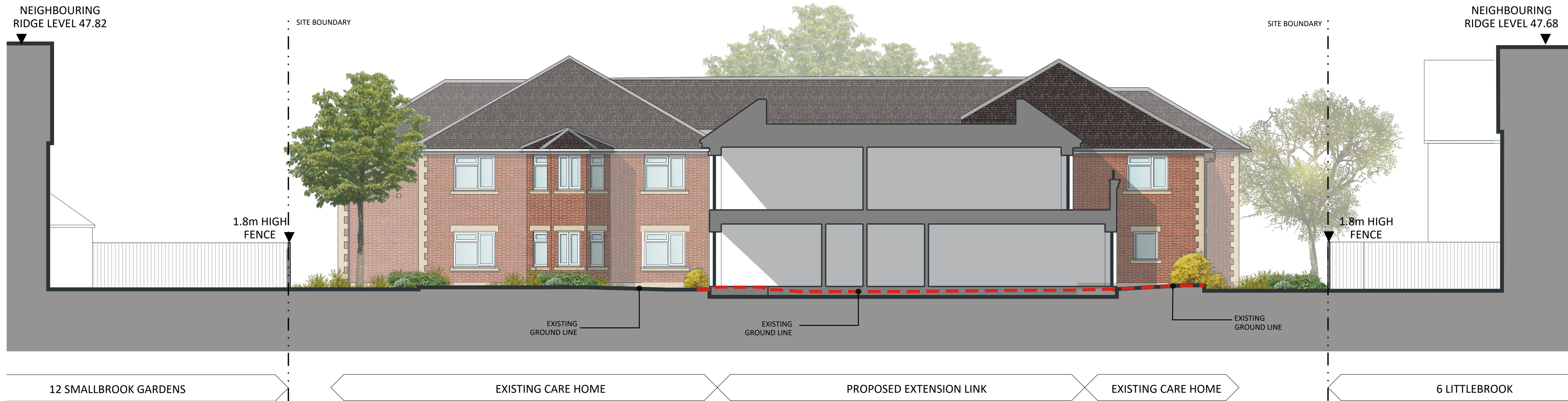
SECTION E
