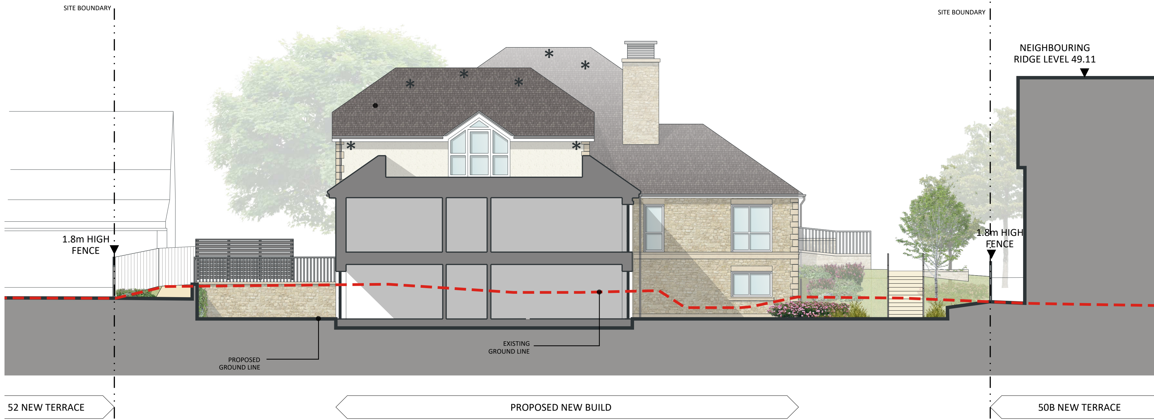
SECTION F
