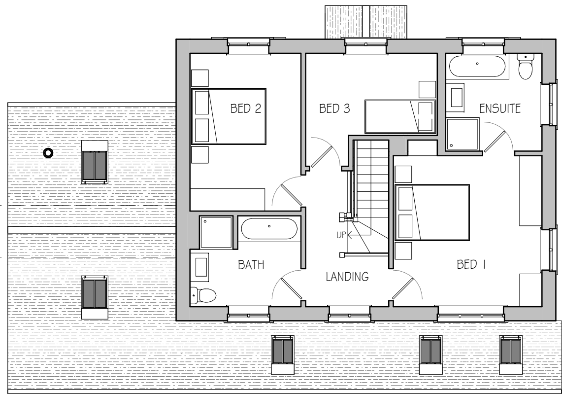
FIRST FLOOR 1 : 100
