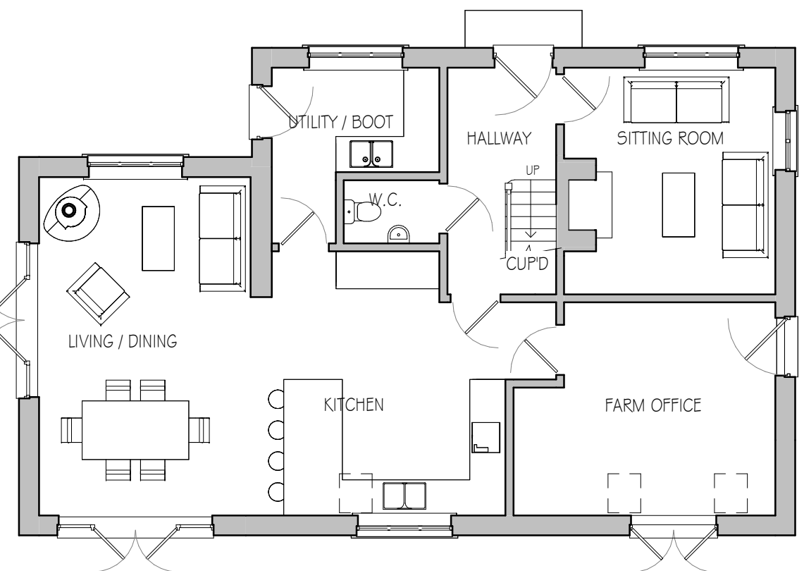
GROUND FLOOR 1 : 100
