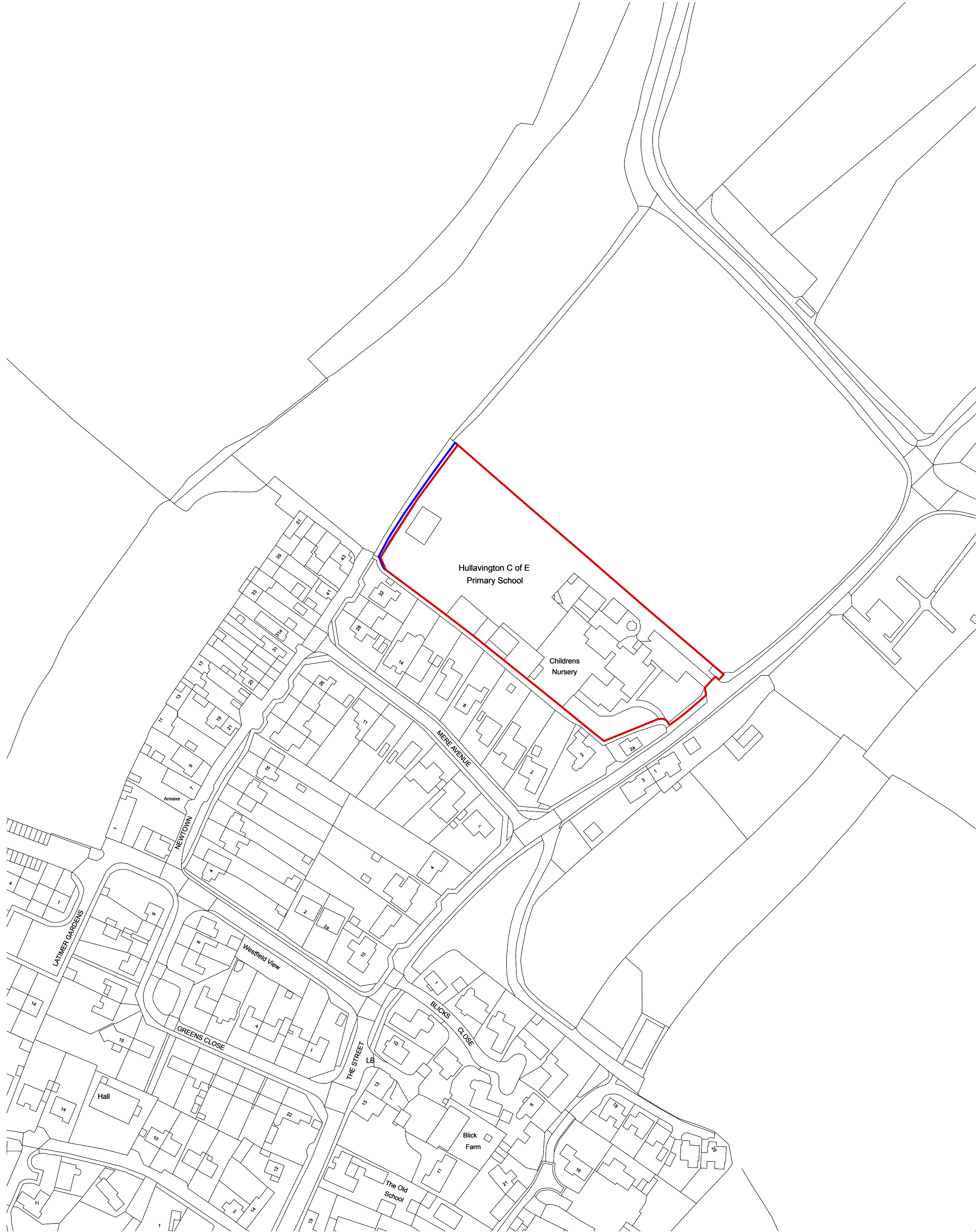
1 Site Location Plan Scale 1:1250
