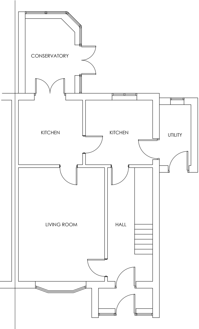
EXISTING FLOORPLAN
