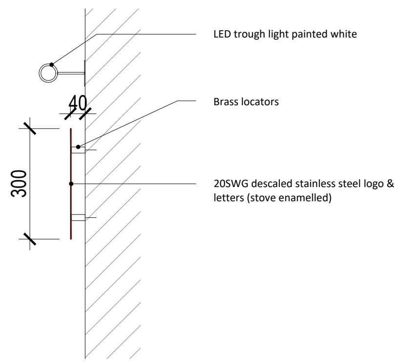
PROPOSED EXTERNAL FASCIA SIGN SECTION DETAIL 1:10 @ A3
