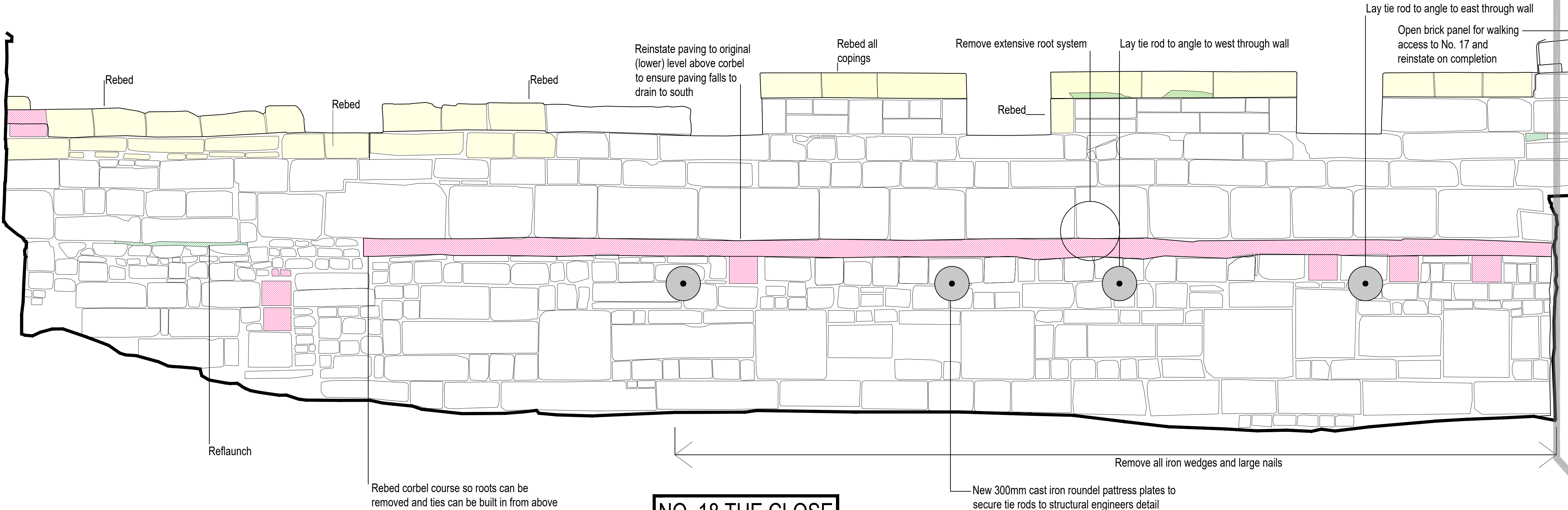
2 NO. 18 THE CLOSE - SOUTH ELEVATION P-04 1:20
