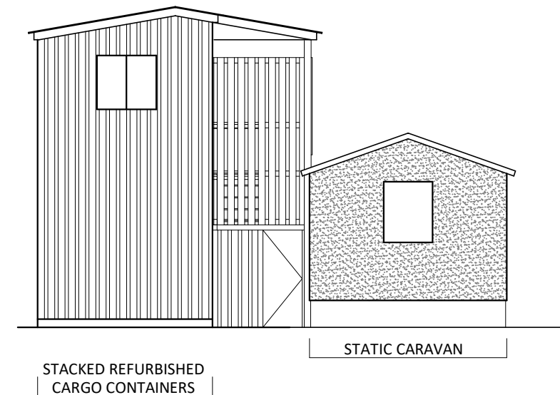
TEMPORARY ACCOMMODATION WEST ELEVATION - SIDE
