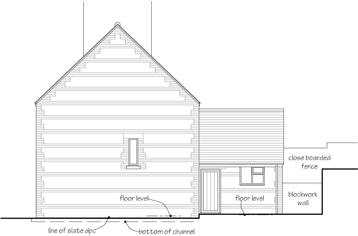
NORTH ELEVATION
