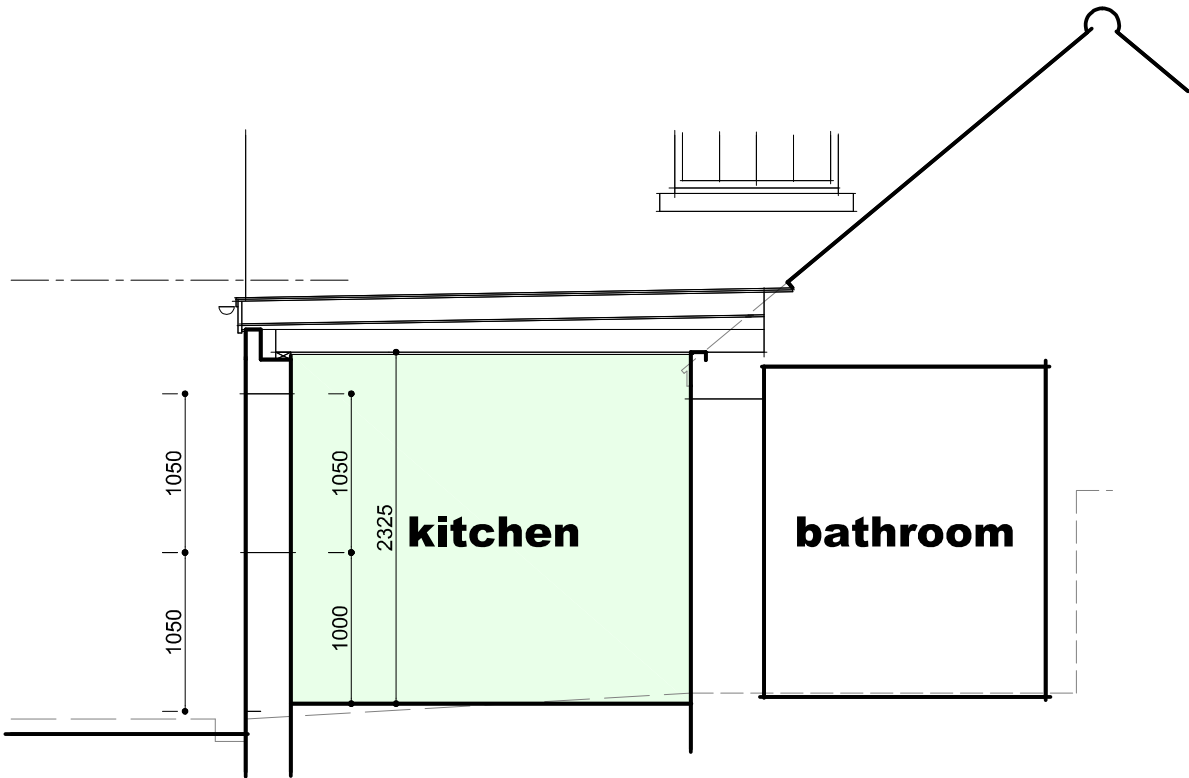
SECTION
