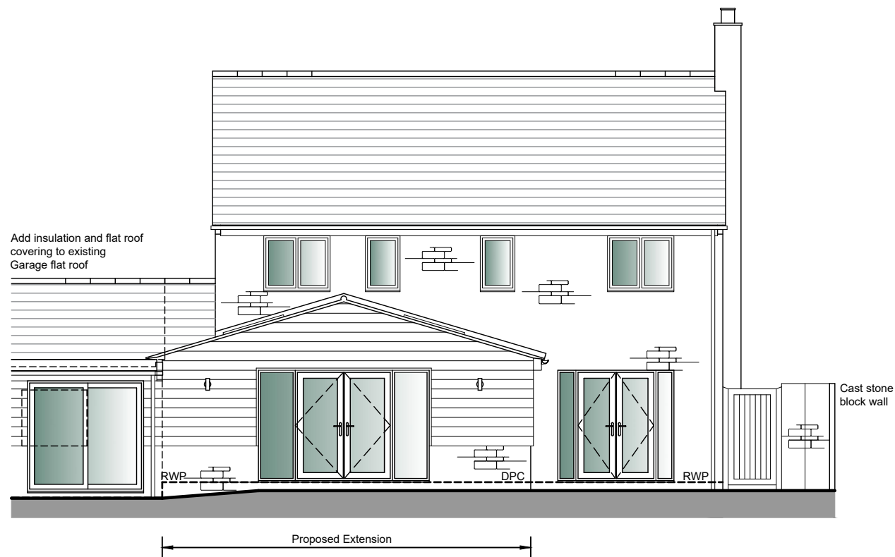
West Elevation
