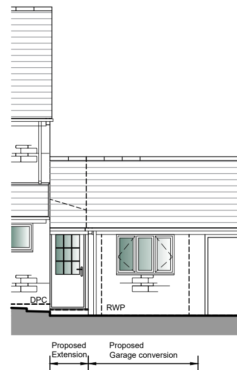
Part East Elevation
