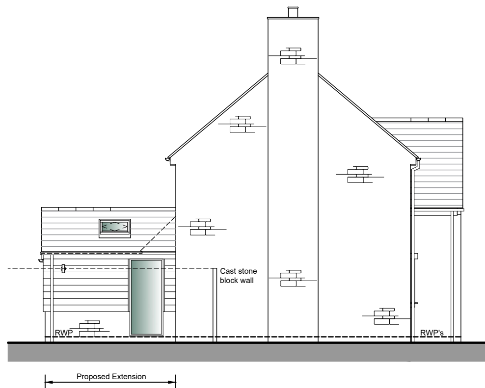
South Elevation
