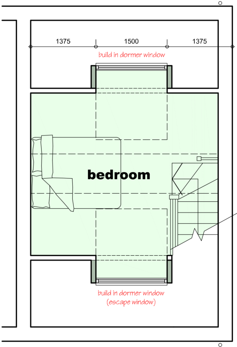
ROOF SPACE PLAN
