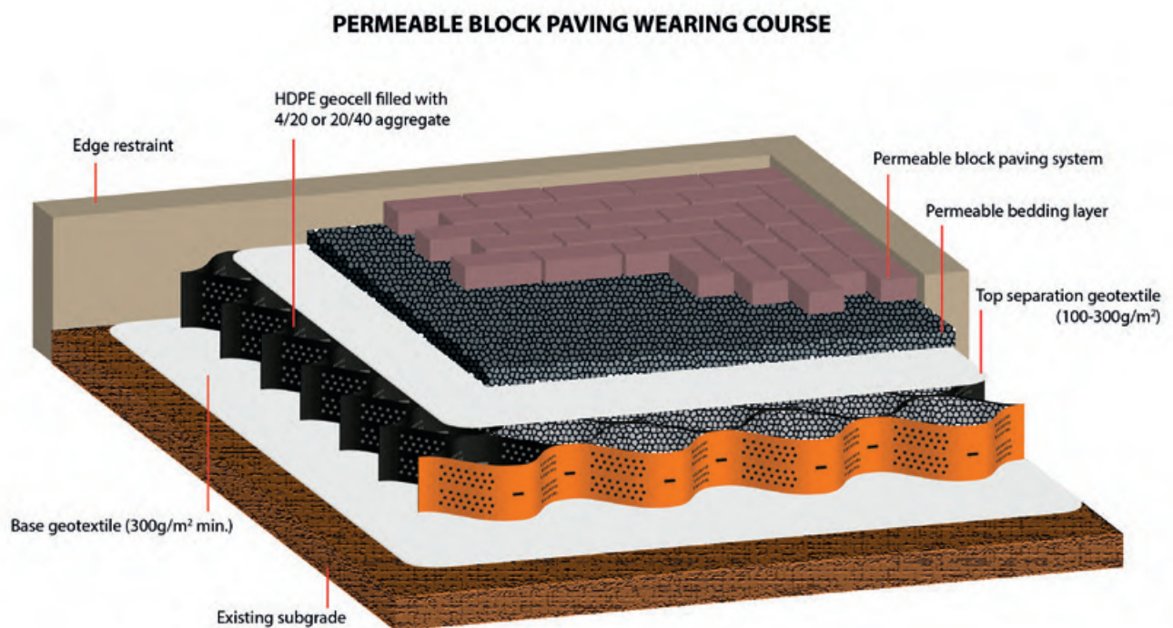
Figure 8: The recommended specification when installing permeable block paving above a cellular confinement system [image courtesy of Core LP].
