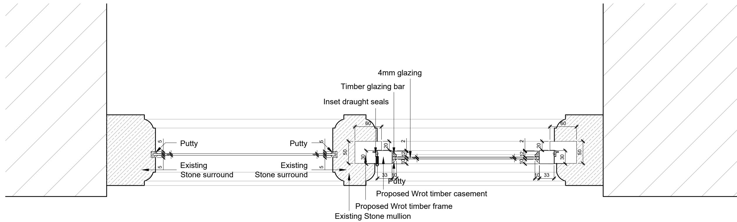
Window Jamb (Direct glazing) 1:5
