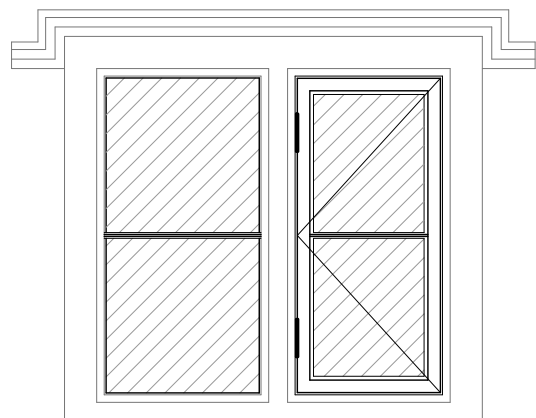
Window WF-01 Elevation - 1:20
