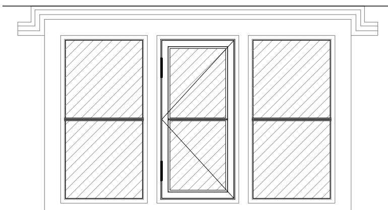
Window WF-05 Elevation - 1:20
