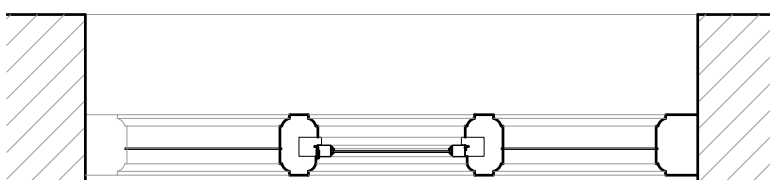
Window WF-04 Plan - 1:20
