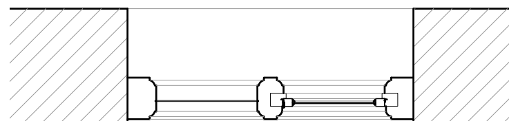
Window WF-02 Plan - 1:20
