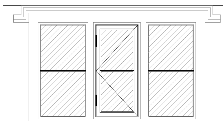
Window WF-03 Elevation - 1:20
