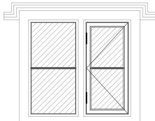
Window WF-02 Elevation - 1:20
